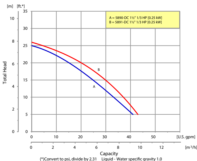
Performance of 12 Volt DC Submersible Pump
