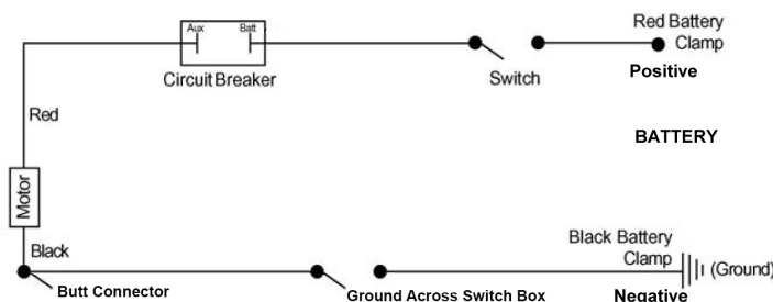
Figure 1 - Wiring Diagram
