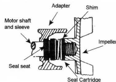
Figure 1 - Mechanical Seal
