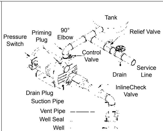
Fig. 4b SHALLOW WELL (WITH INLINE CHECK VALVE)
