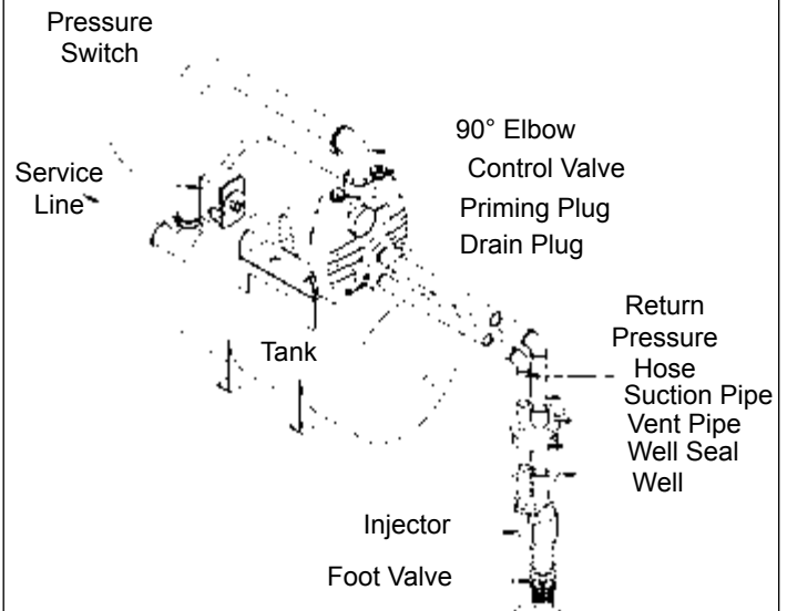
Fig. 4d DEEP WELL - TANK MOUNTED SYSTEM (DOUBLE PIPE INSTALLATION WITH FOOT VALVE)
