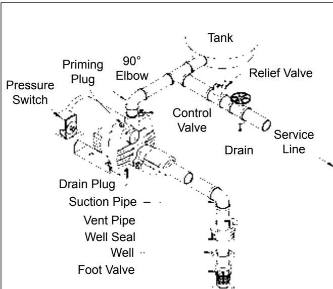
Fig. 4a SHALLOW WELL (WITH FOOT VALVE)
