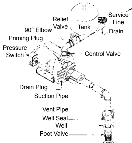
Fig. 4c SHALLOW WELL - INLINE TANK (WITH FOOT VALVE)
