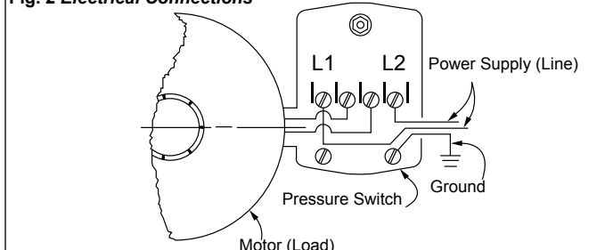
Fig. 2 Electrical Connections
