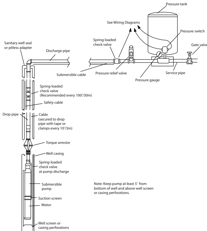
FIGURE 1 Installation Diagram
